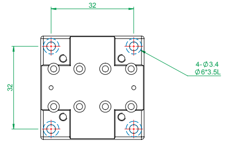
MX(Y)L40-A series bottom plate mounting holes
