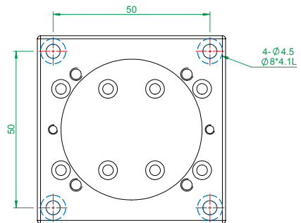
MX(Y)L60-A series bottom plate mounting holes
