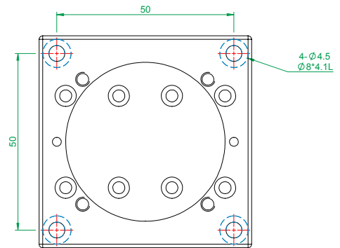
MX(Y)L60-A series bottom plate mounting holes
