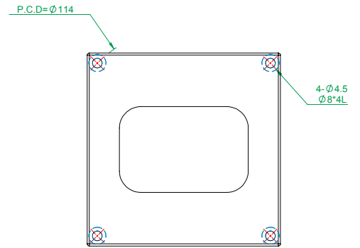
MX(Y)L90-A series bottom plate mounting holes
