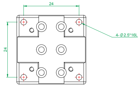
MX(Y)L30-A series bottom plate mounting holes
