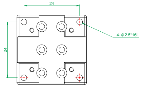
MX(Y)L30-A series bottom plate mounting holes
