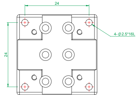
MX(Y)L30-A series bottom plate mounting holes
