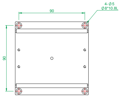
MX(Y)100-S series bottom plate mounting holes
