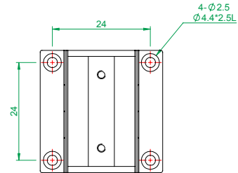
MX(Y)30-S series bottom plate mounting holes
