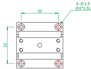
MX(Y)40-S series bottom plate mounting holes
