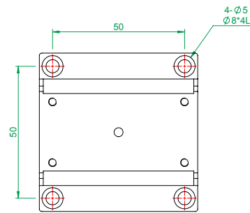
MX(Y)60-S series bottom plate mounting holes
