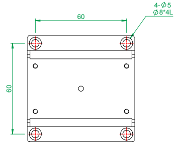
MX(Y)70-S series bottom plate mounting holes
