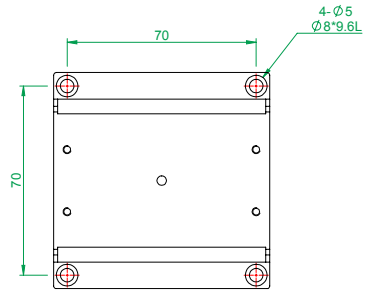
MX(Y)80-S series bottom plate mounting holes
