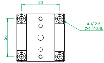
MX(Y)25-S series bottom plate mounting holes
