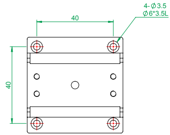
MX(Y)50-S series bottom plate mounting holes
