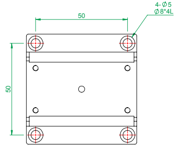
MX(Y)60-S series bottom plate mounting holes
