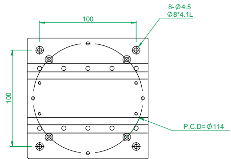
MX(Y)L125-A series bottom plate mounting holes
