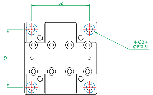
MX(Y)L40-A series bottom plate mounting holes
