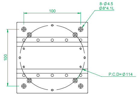
MX(Y)L125-A series bottom plate mounting holes
